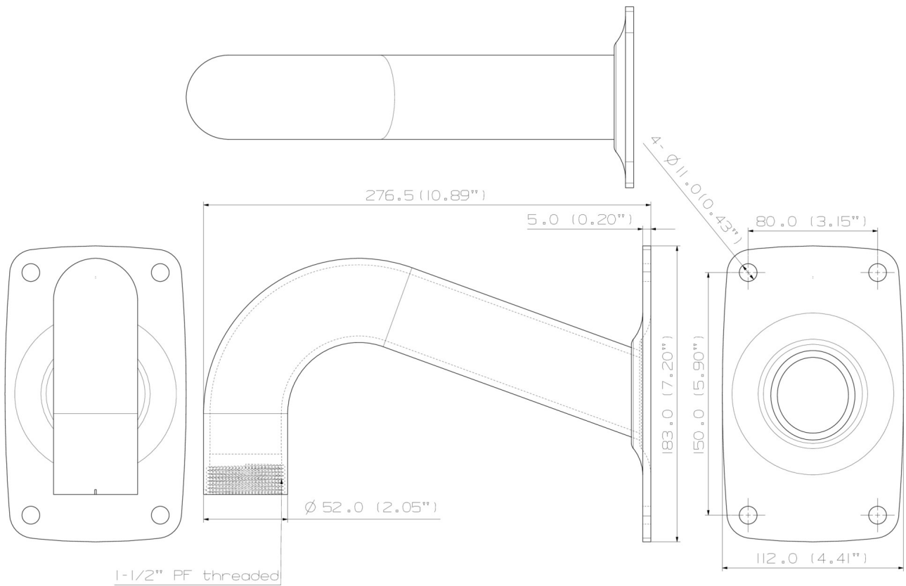
SCX-300WM Unit : mm (inch)
